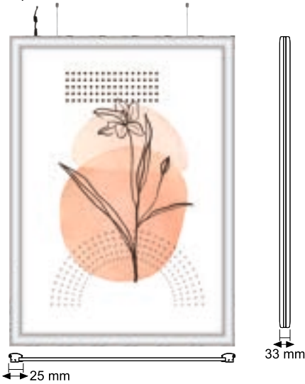
LED Frame 25 mm | LED Leuchtrahmen 25 mm
